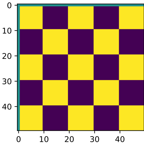
Normalized Linear
