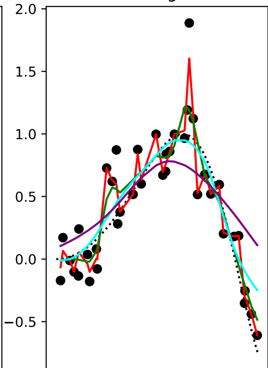
Triweight
