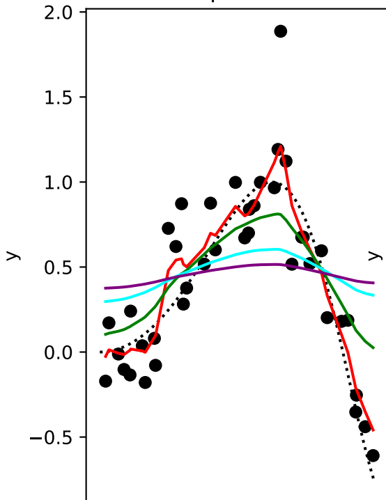
Laplacian
