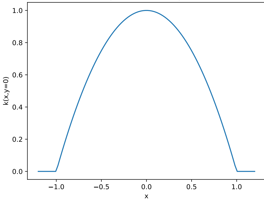
Epanechnikov Shape
