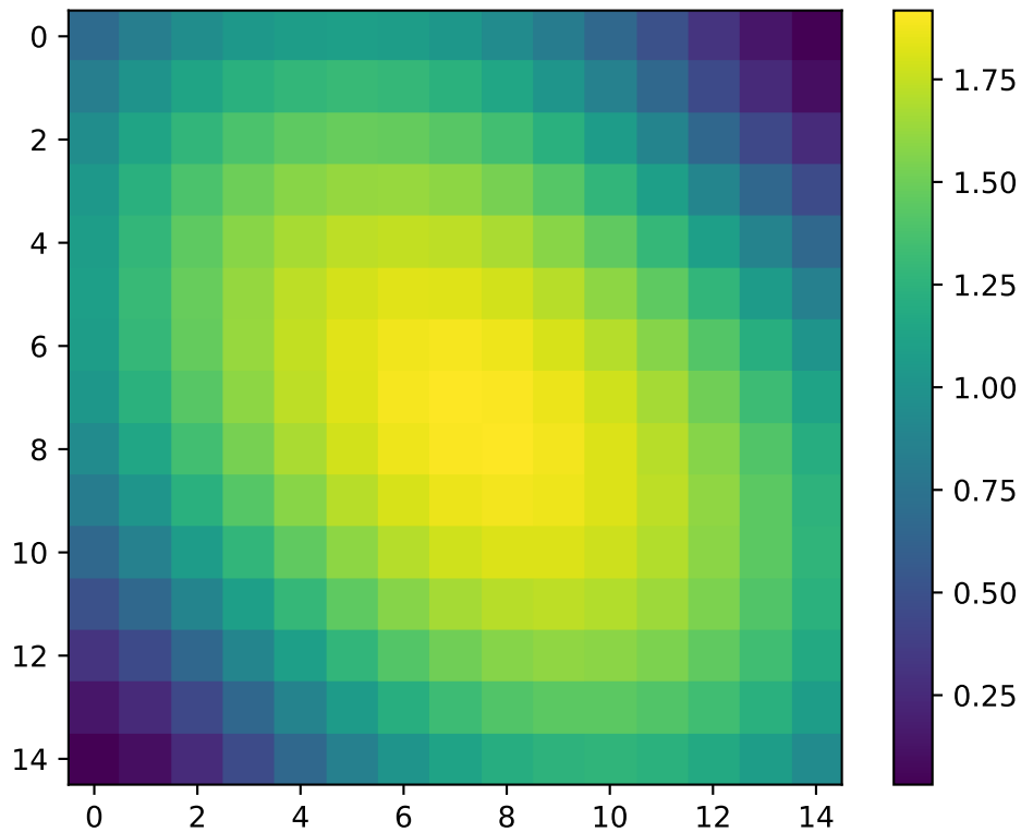
Kernel Matrix
