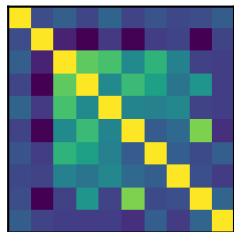
Implicit (out-of-sample)
