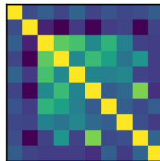
Explicit (out-of-sample)
