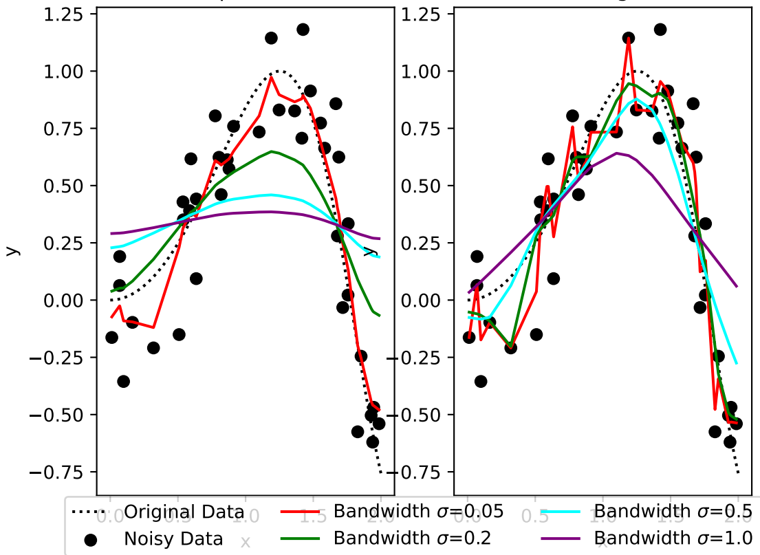
Laplacian
