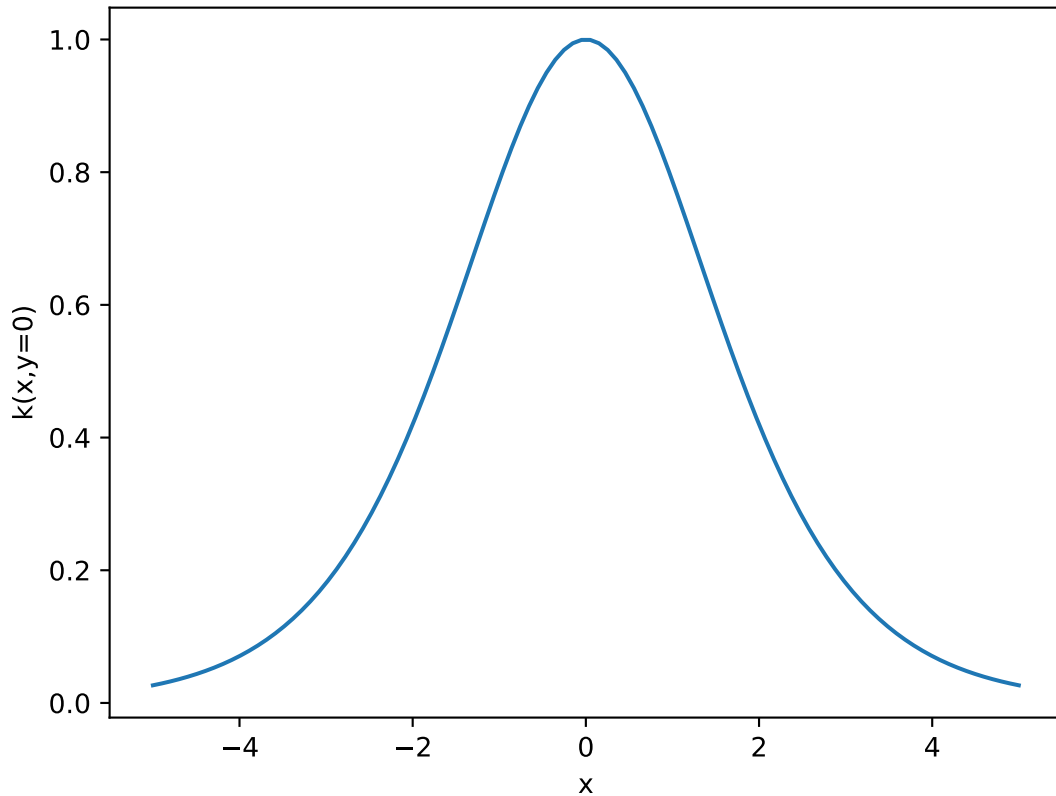
Logistic Shape
