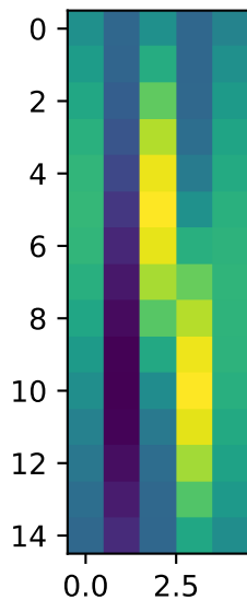
Feature Map
