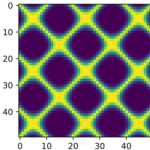
RBF ( \sigma=0.35 )
