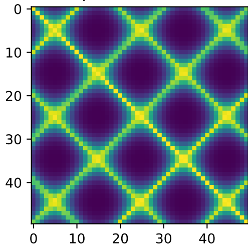
Laplacian ( \sigma=0.35 )
