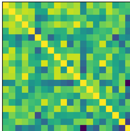
Silverman (Chebyshev)
