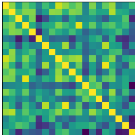
Silverman (Euclidean)
