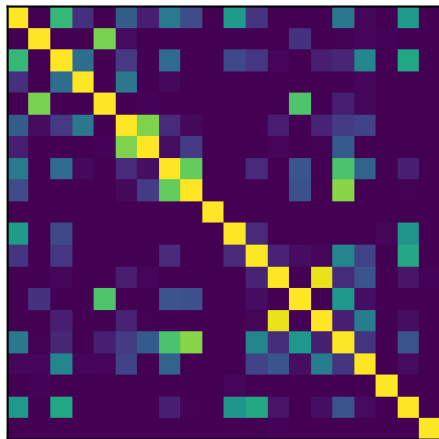
Tricube (Euclidean)
