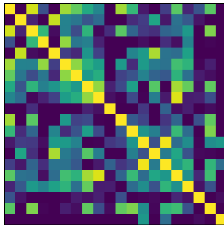
Tricube (Chebyshev)
