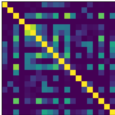
Quartic (Euclidean)
