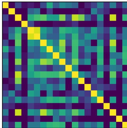
Quartic (Chebyshev)
