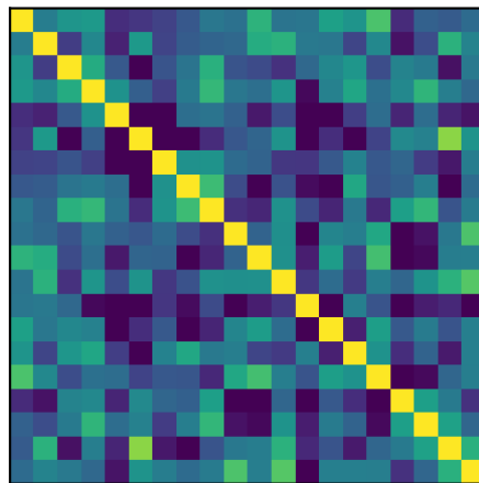
Triangular (Chebyshev)
