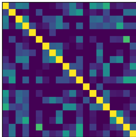
Triangular (Euclidean)
