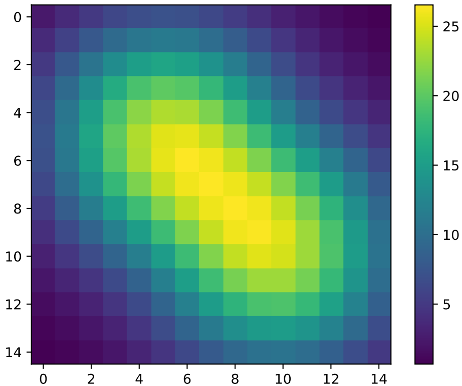
Kernel Matrix
