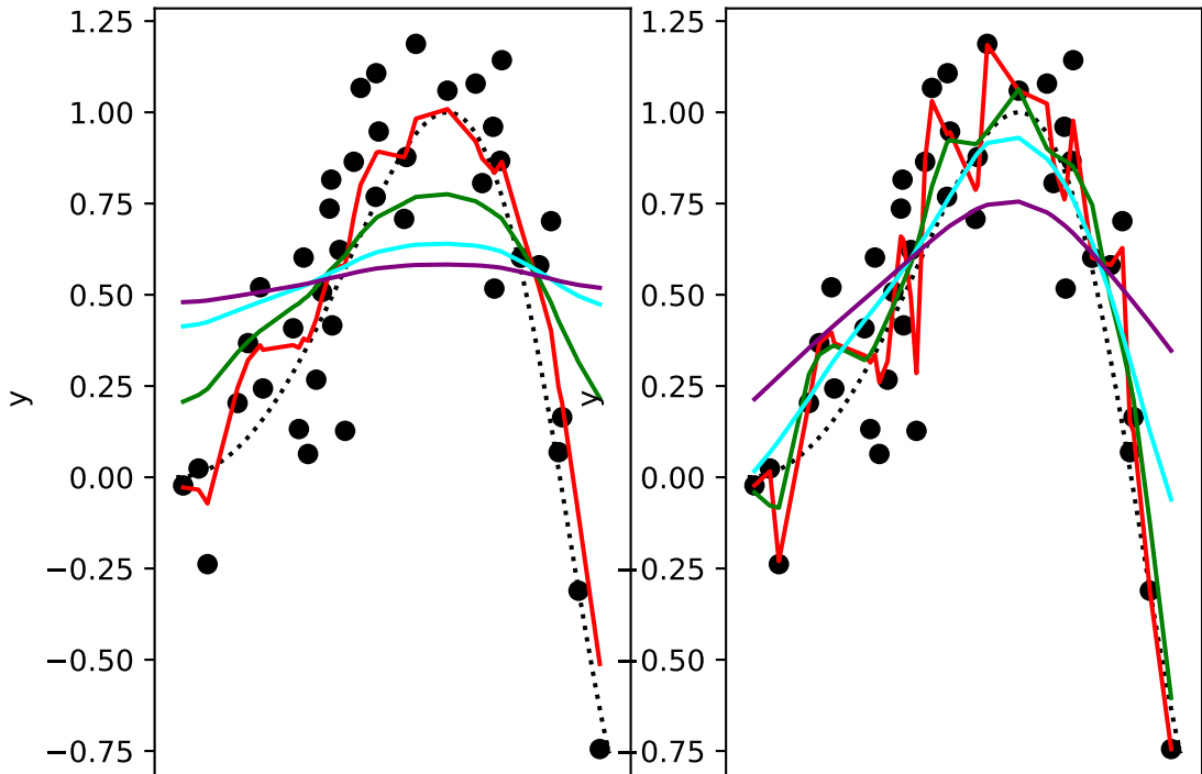
Laplacian
