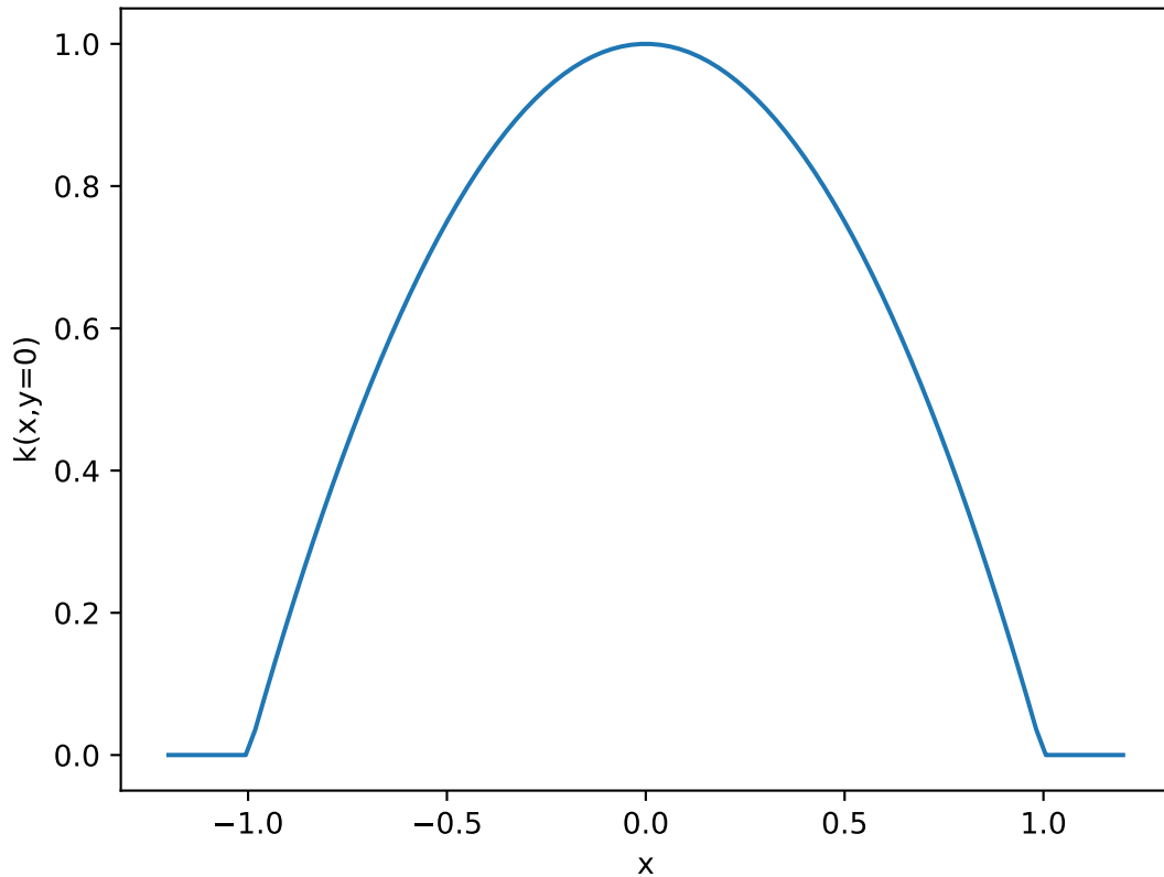
Epanechnikov Shape
